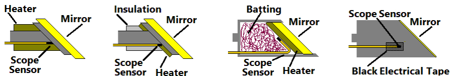
Diagram 1: Sensor placed inside wrap-around heater as close to mirror as possible.
